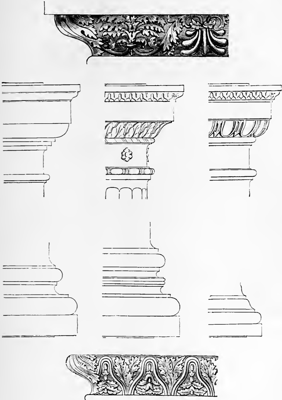
FIG. 150.—MOULDINGS AND ORNAMENTS FROM VARIOUS ROMAN BUILDINGS.
